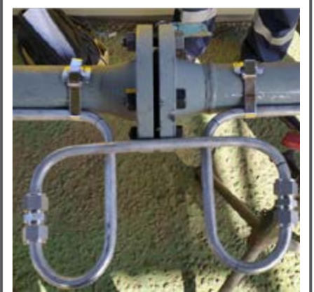
Steam tracing in progress
