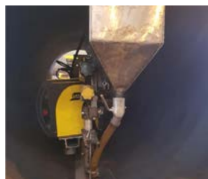
Submerged arc welding (SAW) - 900mm ID
